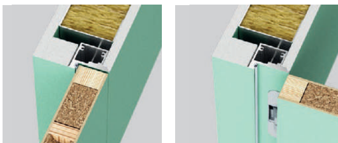
Non-rebated door leaf (outwards) - right door
