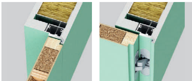
Reversed rebate (opening inwards) - left door
